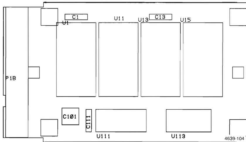
4052R12 16K ROM Pack (670-8201-00) Component Locations.
