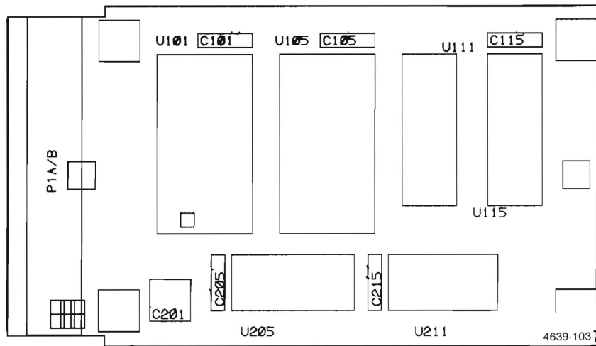
4051R12 8K ROM Pack (670-8200-00) Component Locations.
