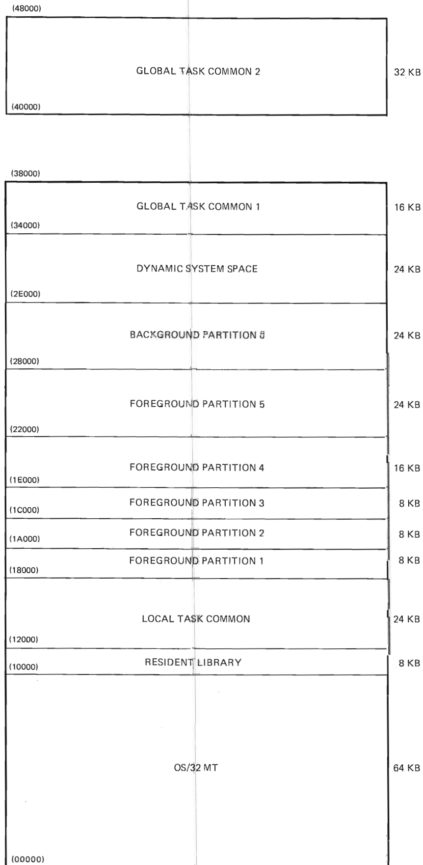
Figure 3-1. OS/32 MT Memory Map Example
