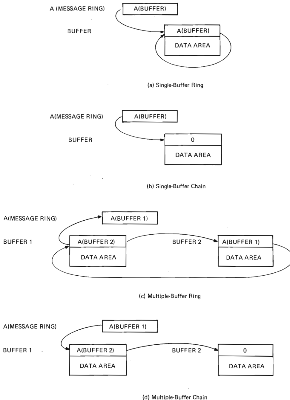
Figure 4-3 Message Buffer Structures
