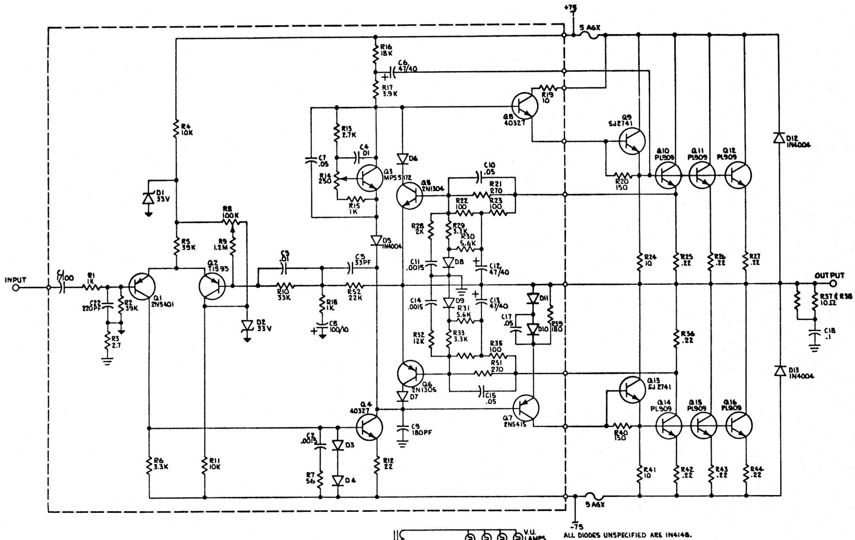
PHASE LINEAR 400 SCHEMATIC DIAGRAM
