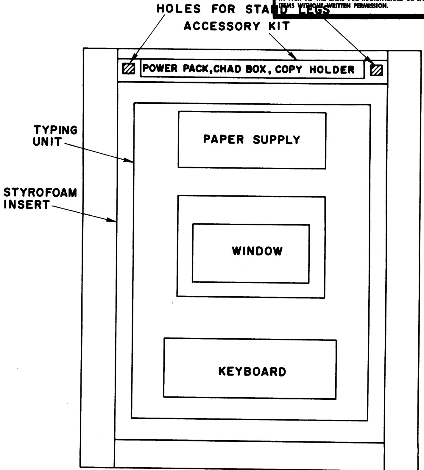
Figure 2-3. Location of Teletype Typing Unit in Carton
