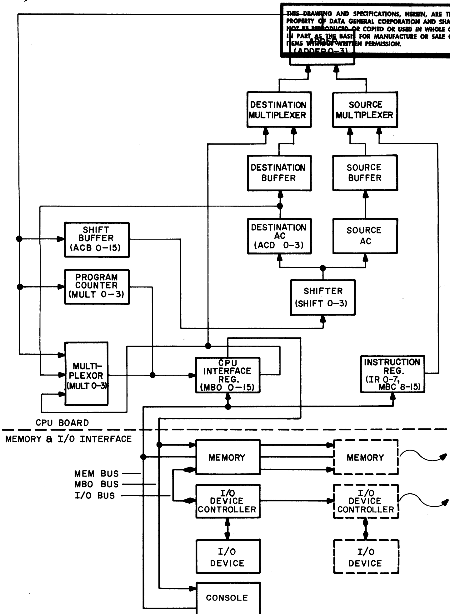
FIGURE I-1 BLOCK DIAGRAM OF NOVA 1200
