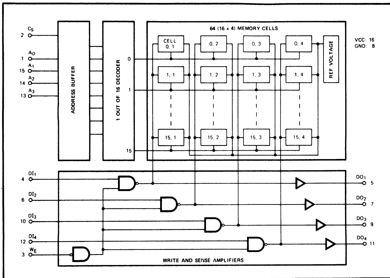
IM5501 Functional Logic Diagram
