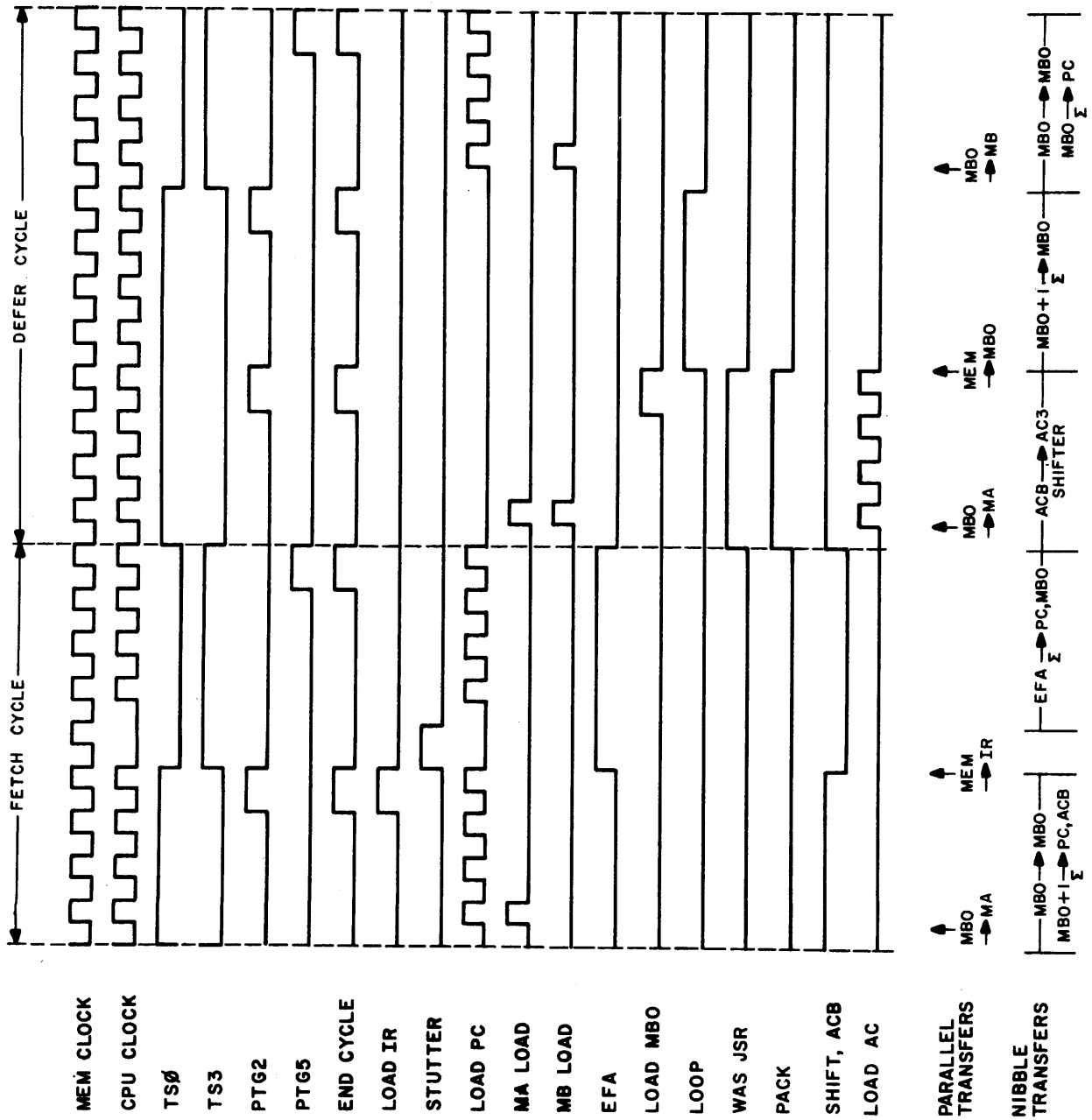
Figure 4-9. JSR @ 20 Timing Diagram
