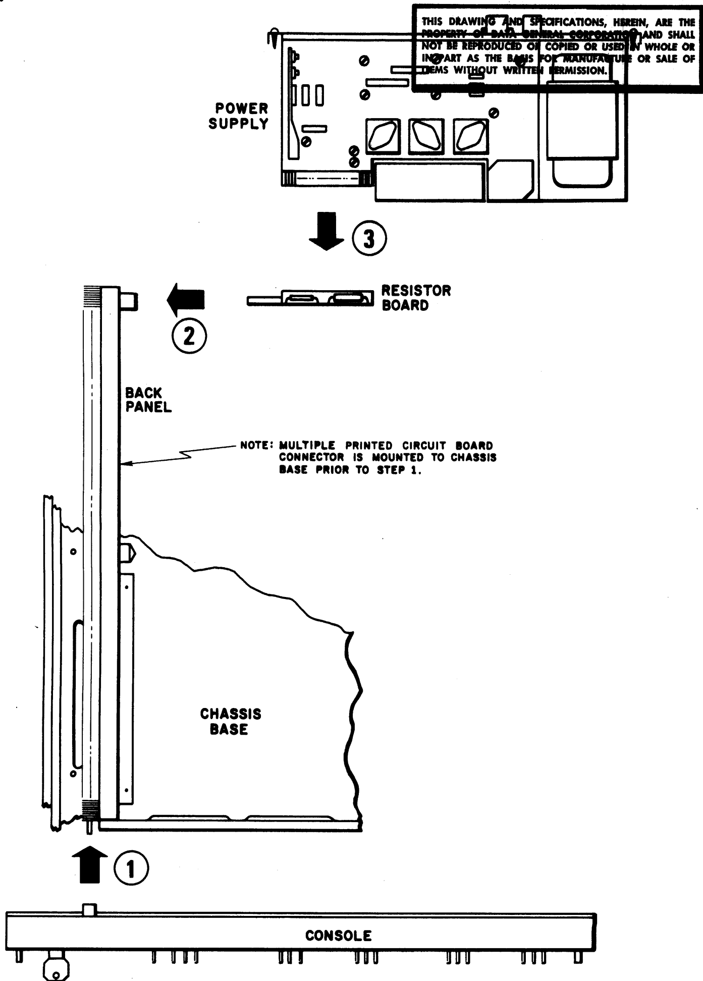
Figure 1-3. Diagram of Plugging Sequence for Assembling the Nova 1200.
