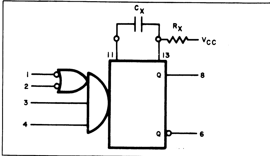
LOGIC DIAGRAM
