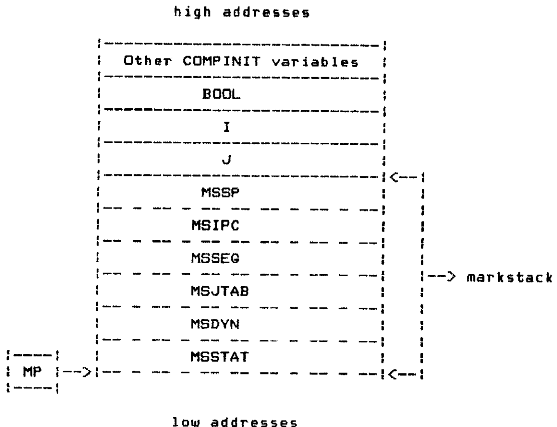
FIGURE 3.5.7. A DATA SEGMENT
