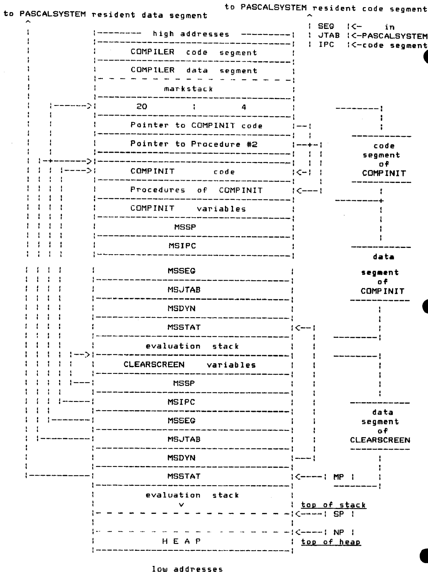
FIGURE 3.5.B. THE STACK DURING CLEARSCREEN
