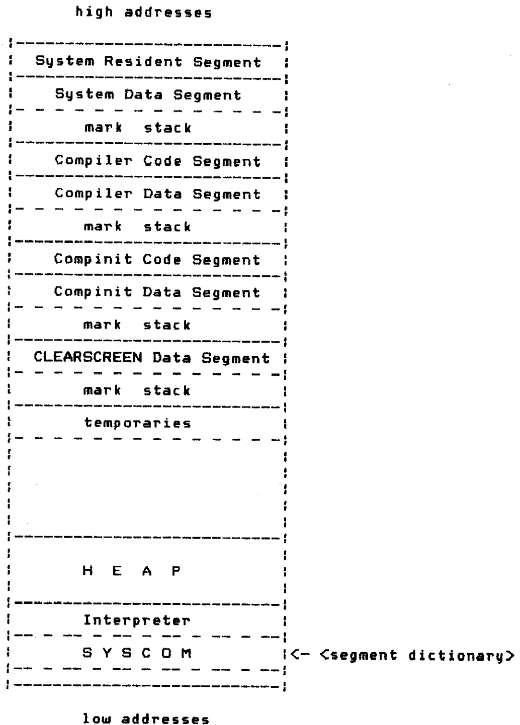
FIGURE 3.5.6. SYSTEM MEMORY DURING CLEARSCREEN EXECUTION
